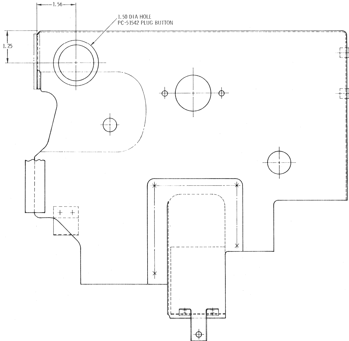
LEFT-HAND FRONT ENGINE COOLING SHROUD PANEL
