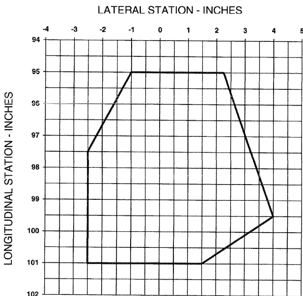
Figure 2-1. Center-of-Gravity Envelope
