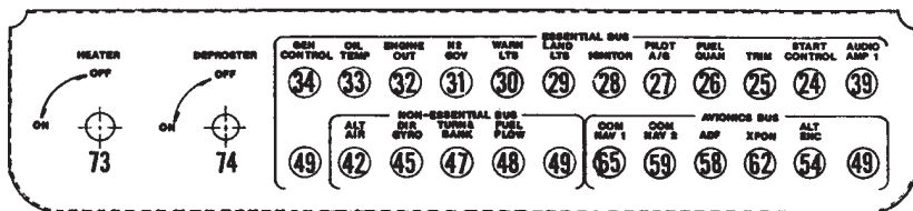
Figure 4-1. Right Seat Pilot in Command Instrument Panel
